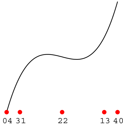
Fig. 2. An adjusted polynomial application of degree 4 that is not injective. Note that control points b_{13} and b_{31} are exchanged.
