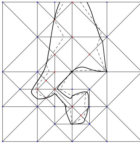
Fig. 9. Polygonization of Taubin's curve (2).
