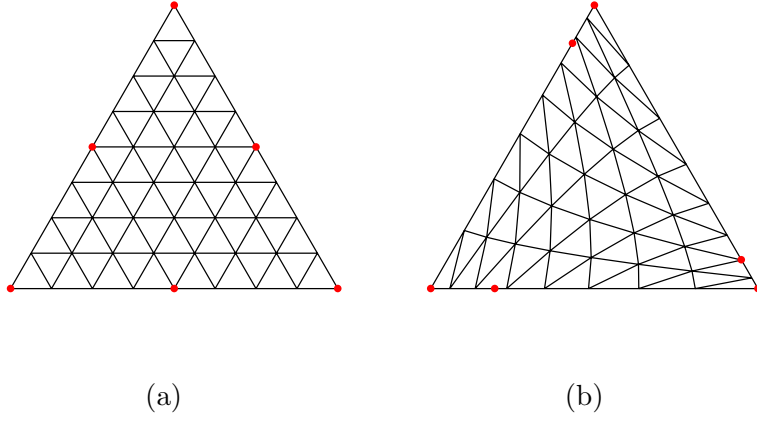
Fig. 3. The action of a quadratic simplicial diffeomorphism: in (a), the control points are in their natural positions, hence the diffeo is the identity; in (b), the control points were moved.
