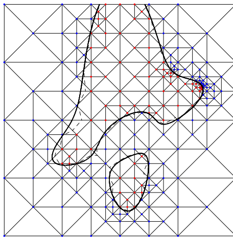
Fig. 10. Polygonization of Taubin's curve (3).
