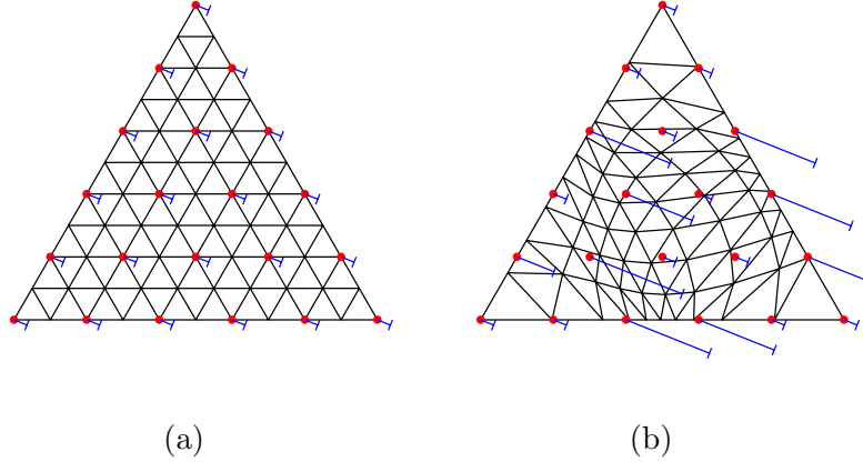
Fig. 5. The action of a rational degree 5 simplicial diffeomorphism: in (a), the control points are in their natural positions and the weights are equal; in (b), the control points are unchanged, but the weights were changed. Note that control points with greater weights are more attractive.
