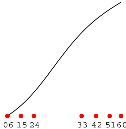
Fig. 1. A degree 6 \Delta^1 -invariant diffeomorphism. Note that the control points are ordered.
