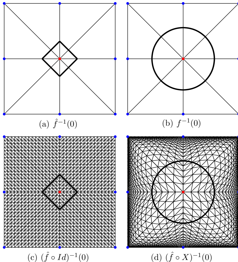
Fig. 6. The zero set of function f(x, y) = x^2 + y^2 - 0.28^2 in four versions: in (a), the linear interpolation over complex K is far from the real curve (b). Composition with the identity changes nothing (c), but a suitable diffeo X deforms the linear interpolation closer to the real curve.
