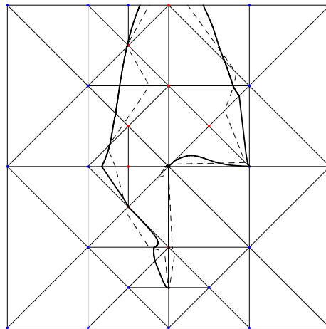
Fig. 8. Polygonization of Taubin's curve (1).
