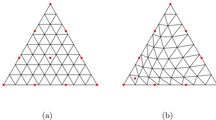
Fig. 4. The action of a cubic simplicial diffeomorphism: in (a), the control points are in their natural positions; in (b), the central control point b_{111} was moved.
